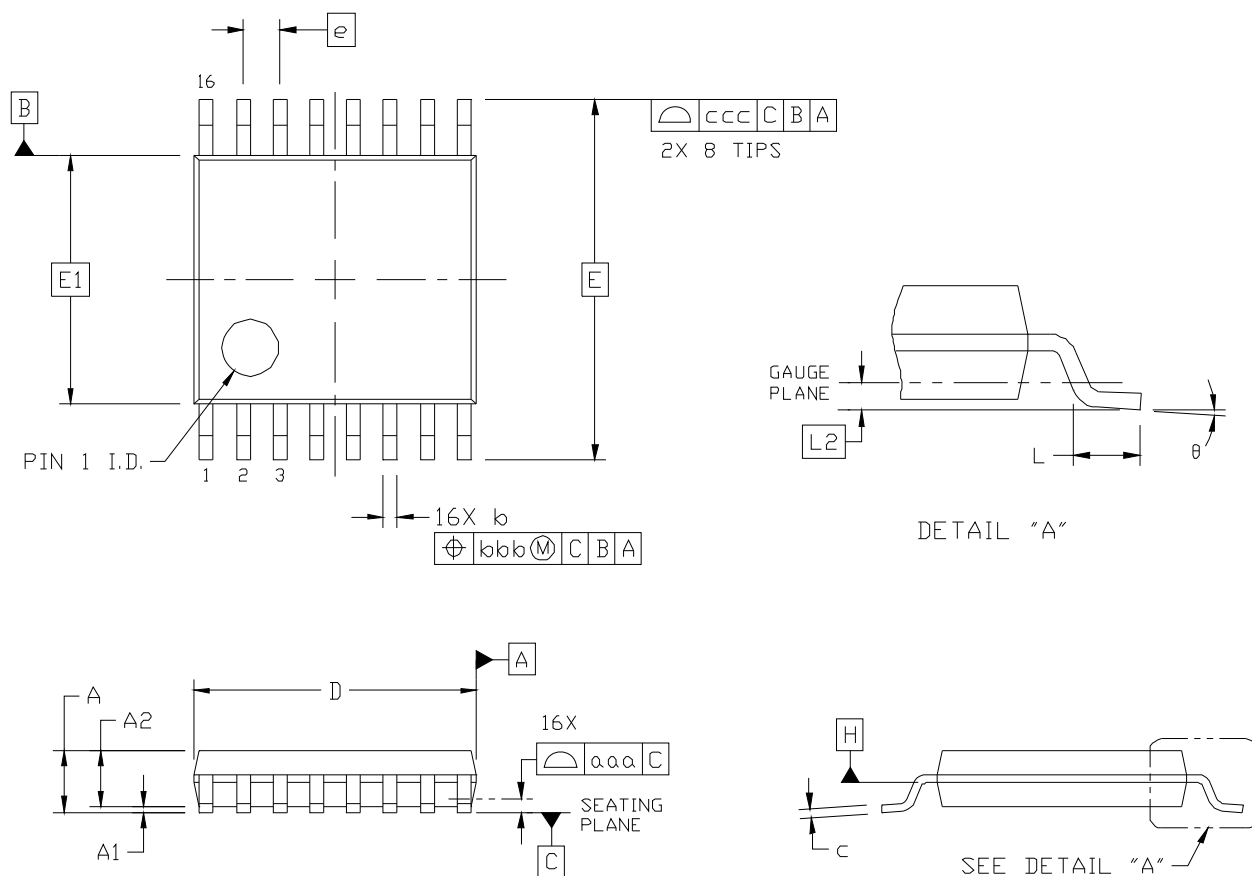
Figure 15. 16-Pin TSSOP
